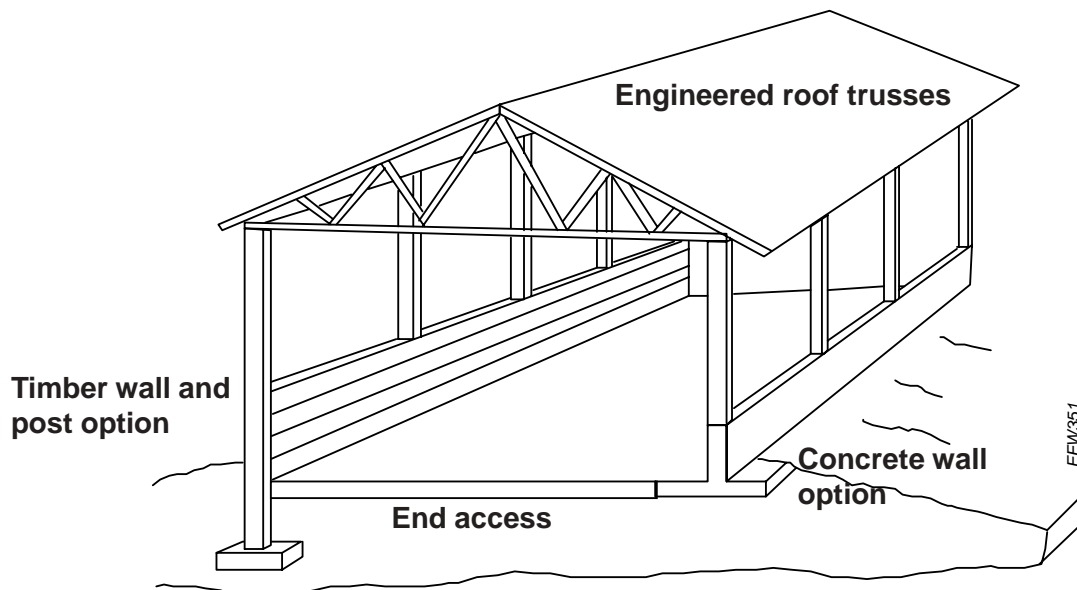
Figure 12. Features of large, roofed, solid-manure storage.
