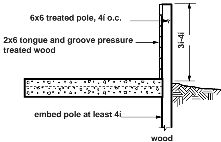
Figure 10. Bucking wall options. Note: These drawings are general representations and are not meant as construction drawings. A site-specific design is recommended in all cases. If soil backfill is to be placed behind the wall, a more economical wall may be possible. [Adapted from Livestock Waste Facilities Handbook , MWPS-18.]
