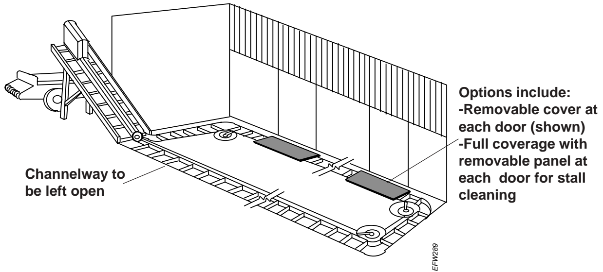
Figure 6. Automated barn cleaner. [Adapted from Livestock Waste Facilities Handbook , MWPS-18.]
