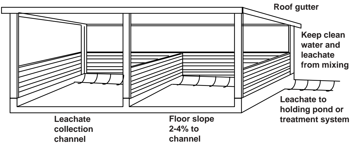
Figure 13. Covered storage with leachate collection for wet materials.
