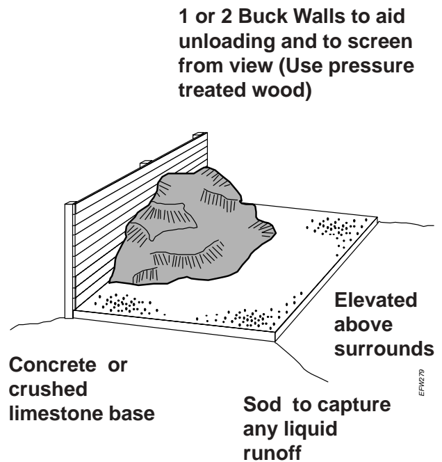
Figure 8. Simple manure stockpile pad, with backstop, that is suitable for a small stable. It is recommended that a tarp or other cover be used to minimize leachate production from precipitation.
