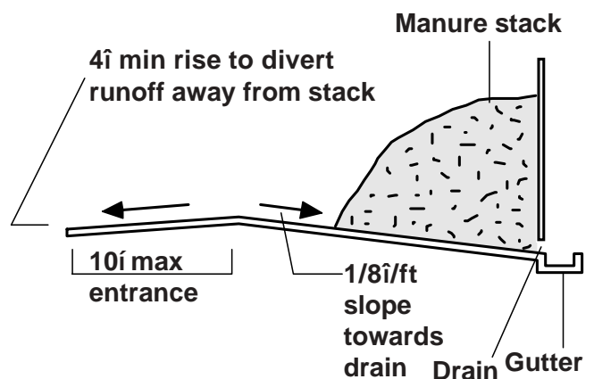
Figure 9. Manure pad slope and drainage. Drain and gutter are recommended in all cases. They are essential if the manure stack will not be protected from rainfall. Leachate (effluent) must be directed to a storage tank and/or suitable method of disposal. [Reproduced with permission from Livestock Waste Facilities Handbook , MWPS-18.]
